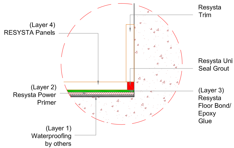
CORNER END PLATE JOINT DETAILS
