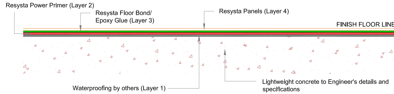
LONGITUDINAL SECTION (Floor)
