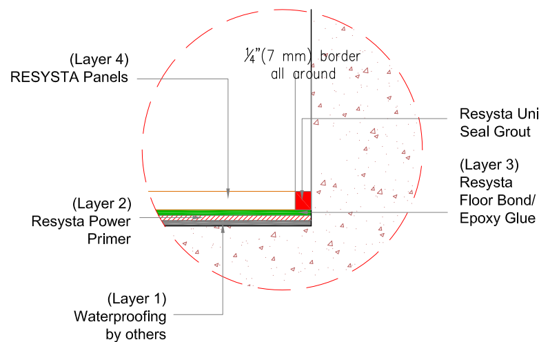
CORNER EXPANSION JOINT DETAILS
