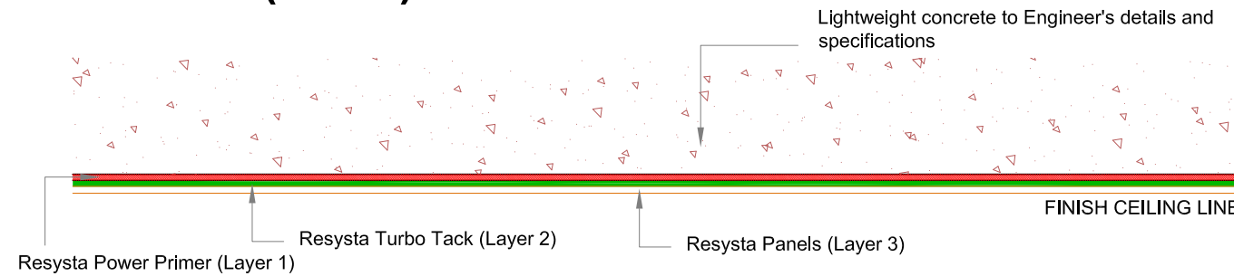
LONGITUDINAL SECTION (Floor)
