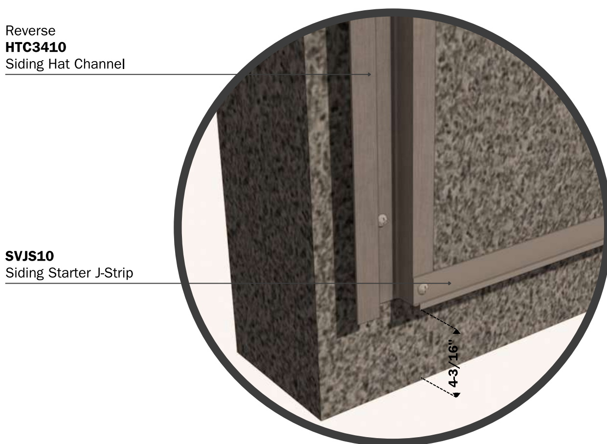
DETAIL Siding Starter J-Strip Deco Profile Quik-Trim System
