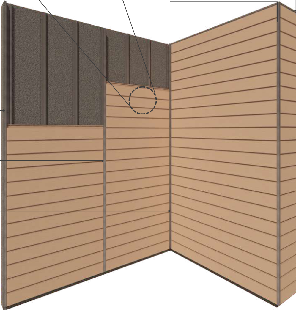
ISOMETRIC VIEW Basic Parts of Deco Profile Quik-Trim System
