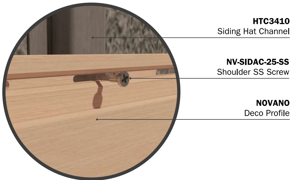
DETAIL Deco Profile Quik-Trim System
