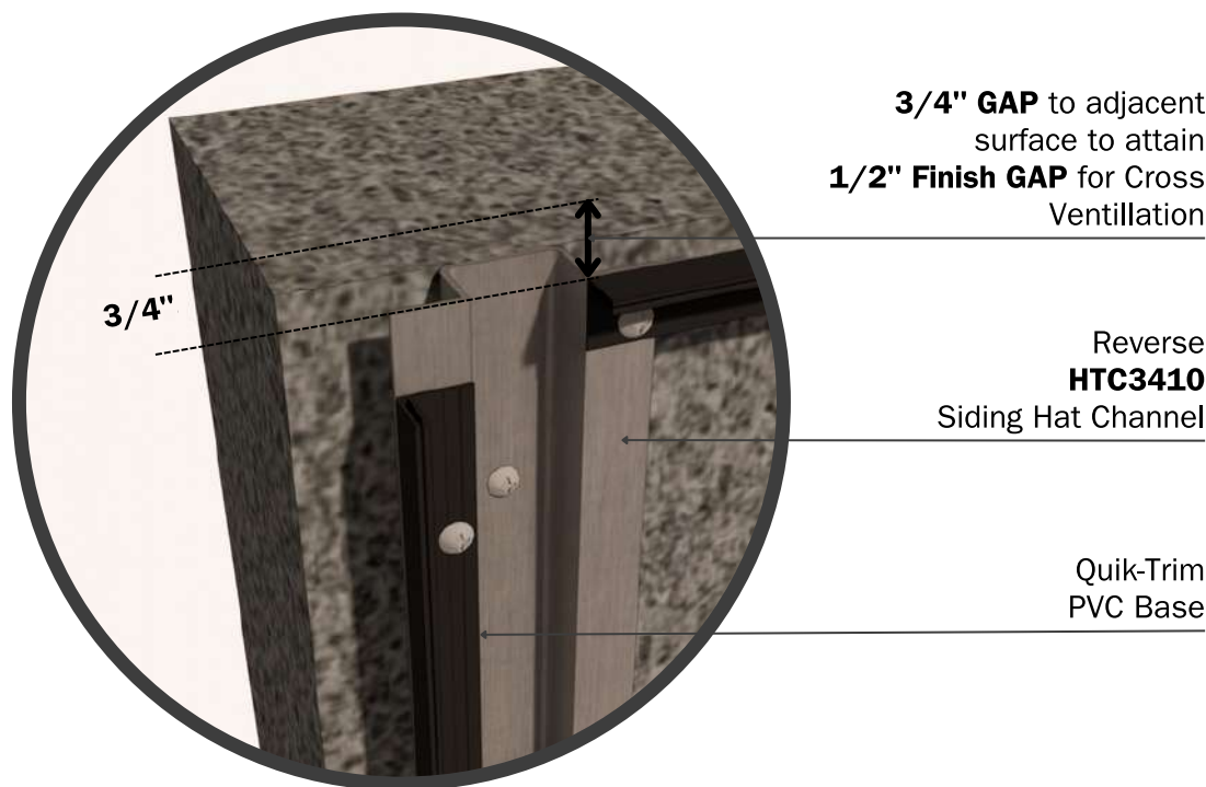
DETAIL PVC Base Deco Profile Quik-Trim System
