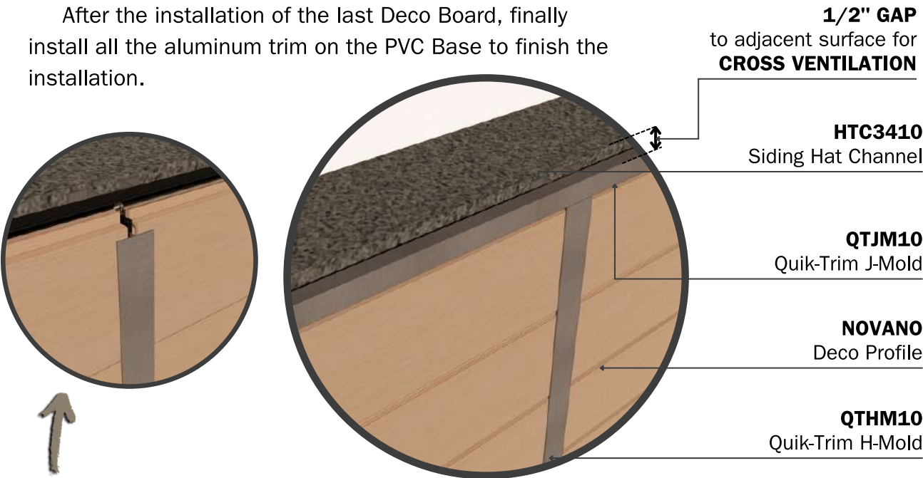
DETAIL Deco Profile Quik-Trim System
