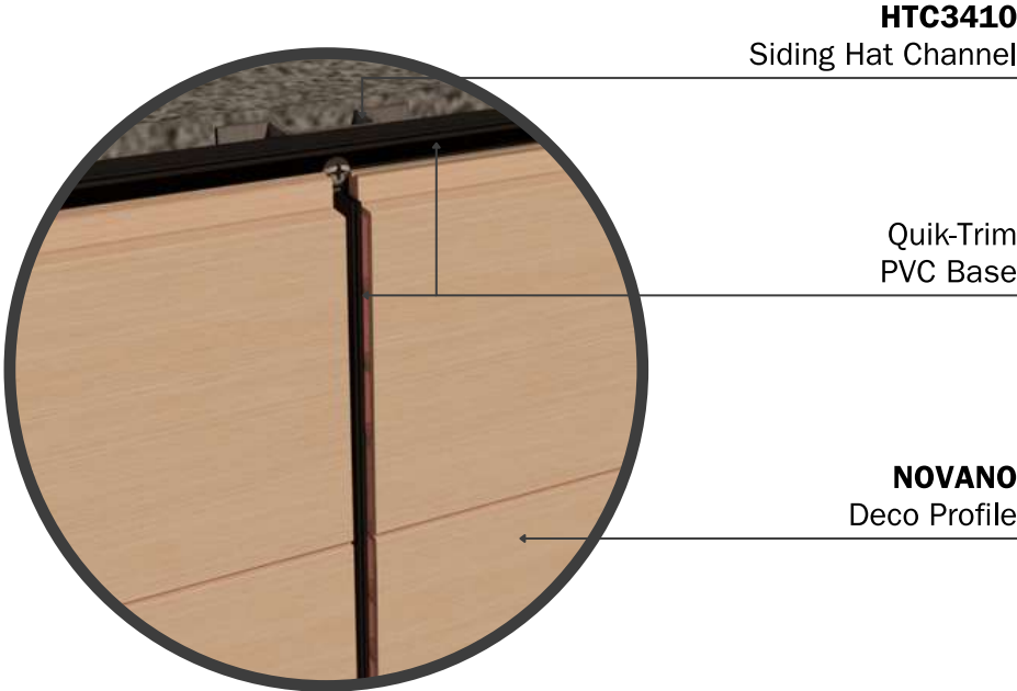
DETAIL Deco Profile Quik-Trim System
