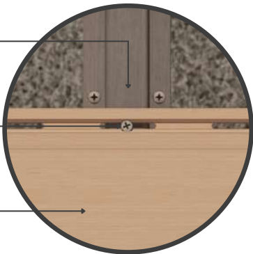
DETAIL Deco Profile Quik-Trim System
