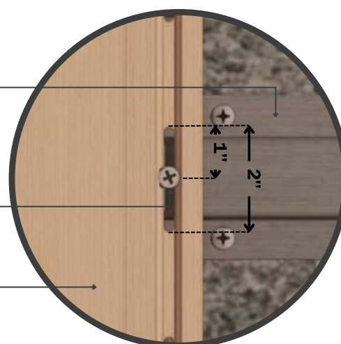
FRONT ELEVATION Deco Profile Quik-Trim System
