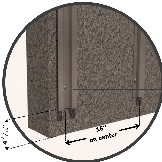
DETAIL Substructure
