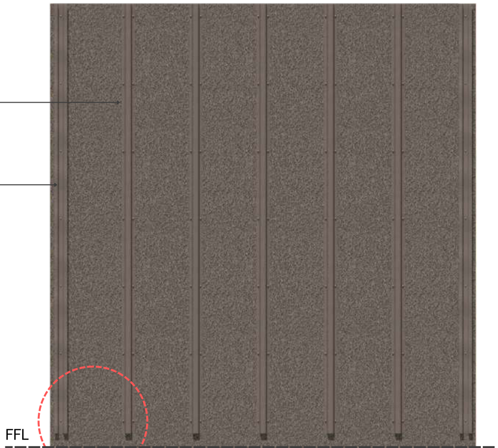
FRONT ELEVATION Substructure Siding 12" Quik-Trim System
