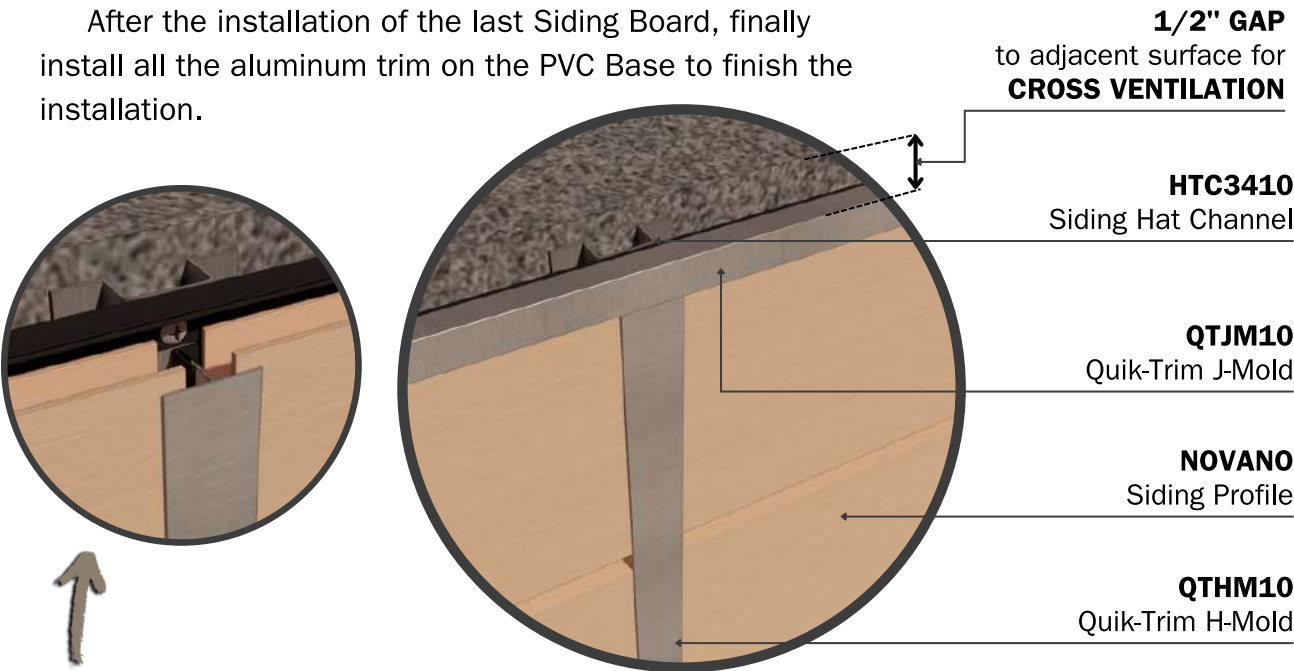
DETAIL Siding 12" Quik-Trim System
