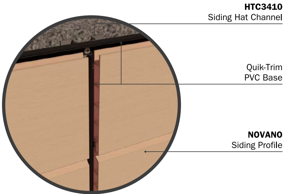
DETAIL Siding 12" Quik-Trim System
