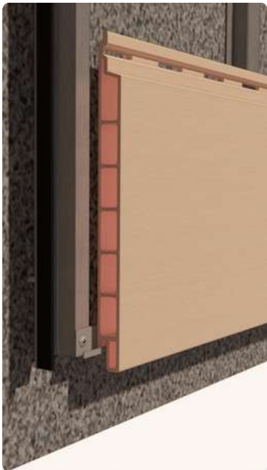
DETAIL 3 Push the NOVANO Siding Board perpendicular into the runner and screw direct to the groove.
