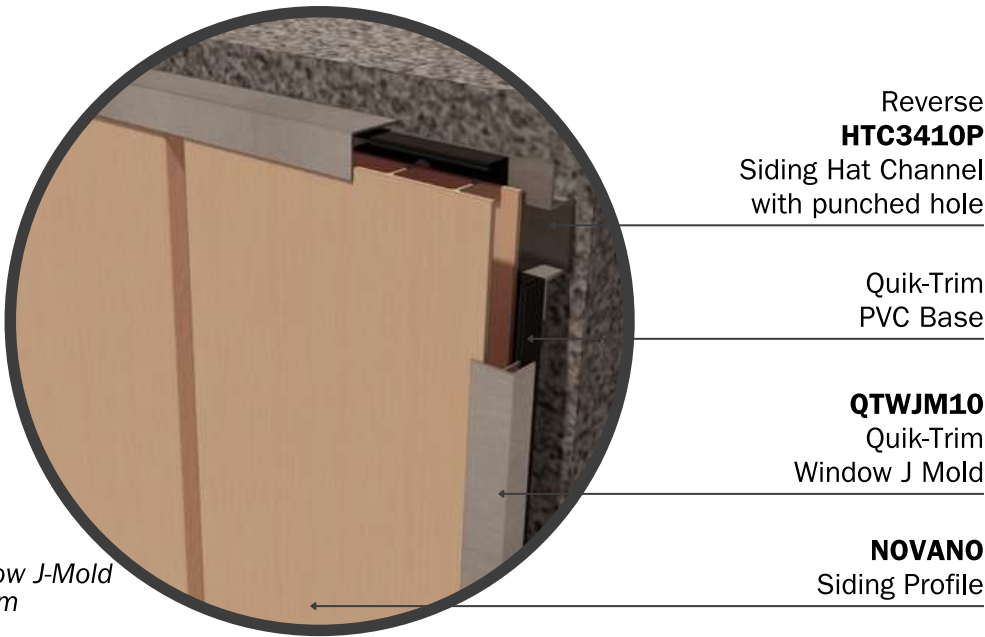
DETAIL Quik-Trim Window J-Mold Quik-Trim System
