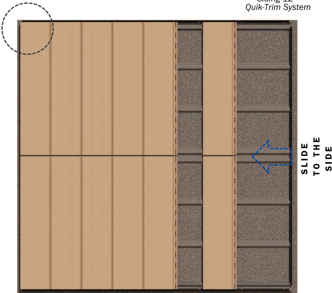
FRONT ELEVATION Siding 12" Quik-Trim System
