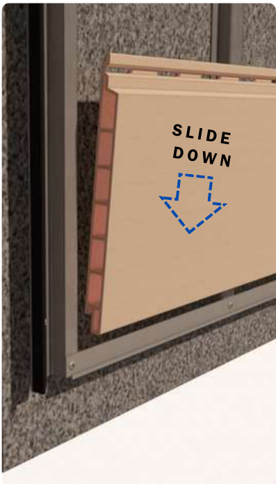
DETAIL 1 Slide down the first NOVANO Siding Board into Siding Starter J-Strip.
