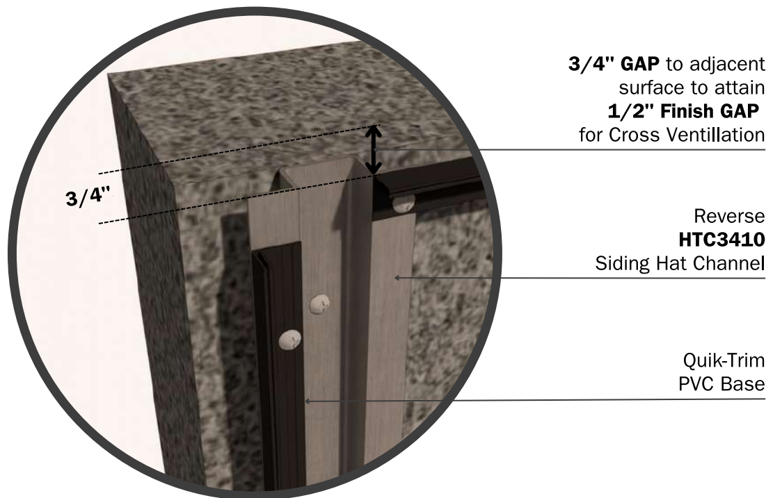
DETAIL PVC Base Siding 12" Quik-Trim System
