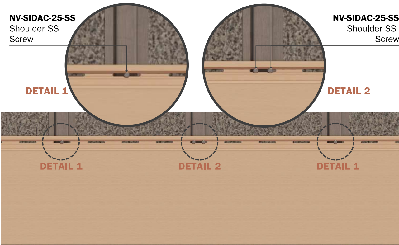
FRONT ELEVATION Siding 12" Quik-Trim System
