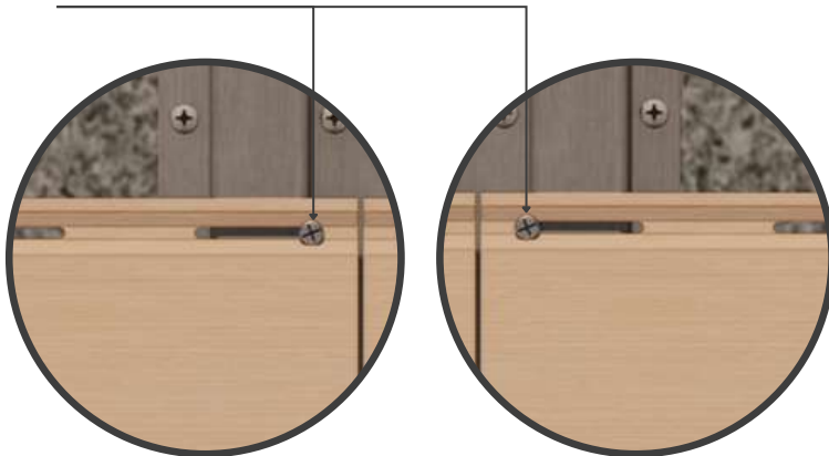
DETAIL Siding 6" & 4" Quik-Trim System
