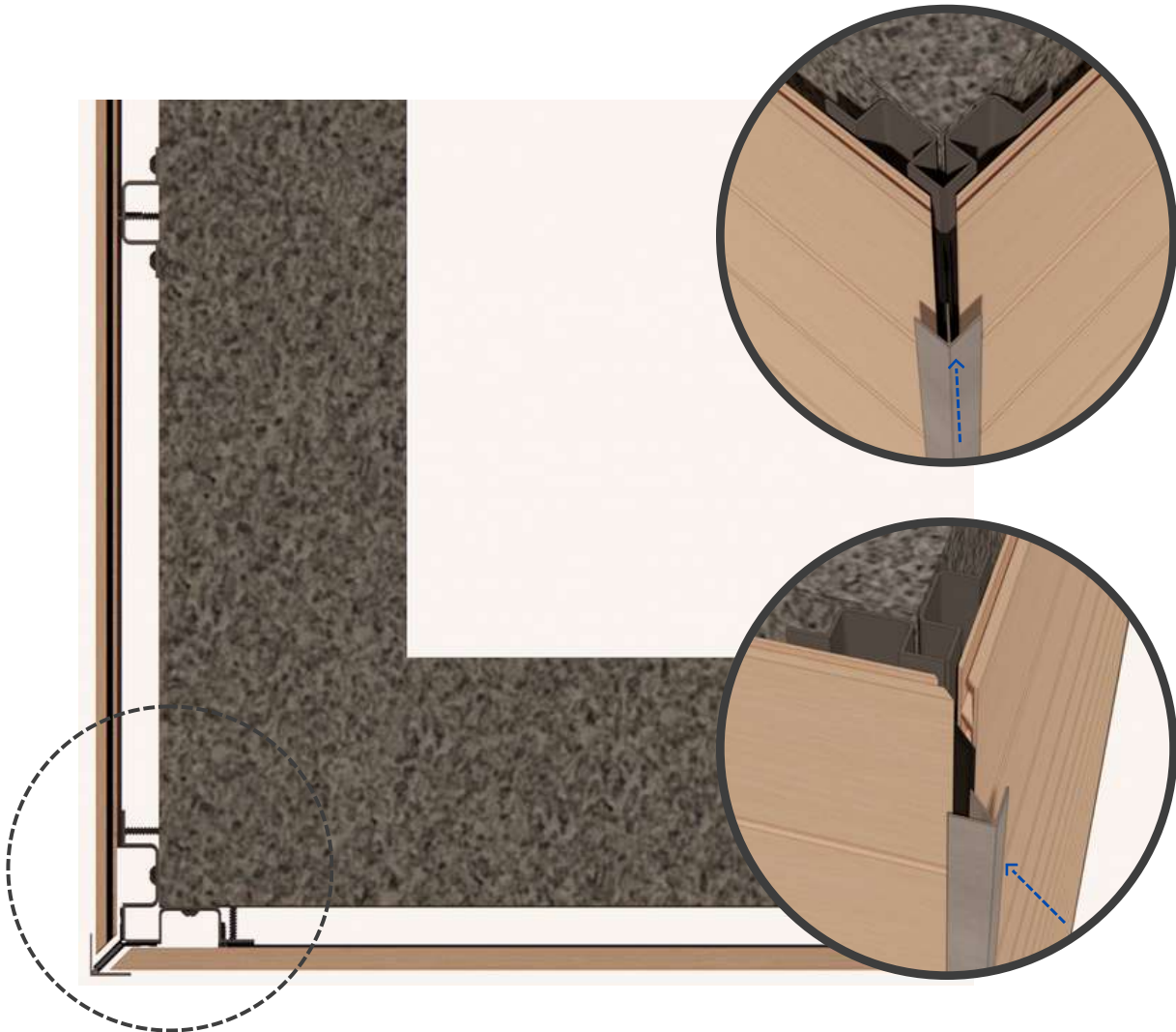
TOP VIEW Outside Corner Quik-Trim System
