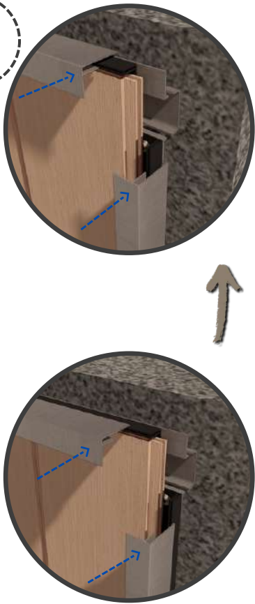
Install the Quik-Trim J-Mold & Quik-Trim Windows J-Mold into the PVC Base
