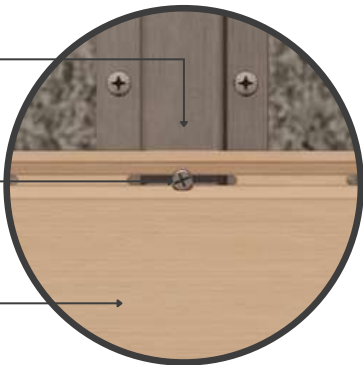
DETAIL Siding 6" & 4" Quik-Trim System
