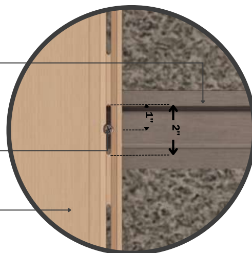
FRONT ELEVATION Siding 6" & 4" Quik-Trim System
