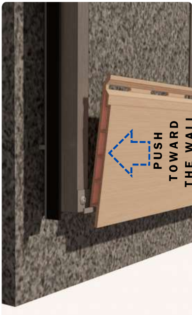
DETAIL 2 Hook the groove end of the first NOVANO Siding Board into the Siding Starter J- Strip with SS screw.
