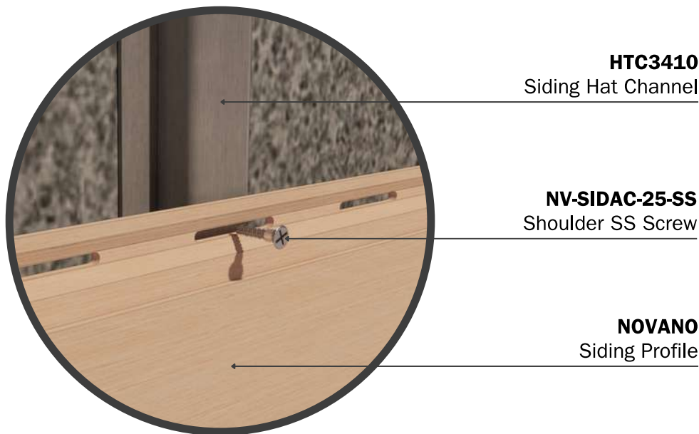
DETAIL Siding 6" & 4" Quik-Trim System
