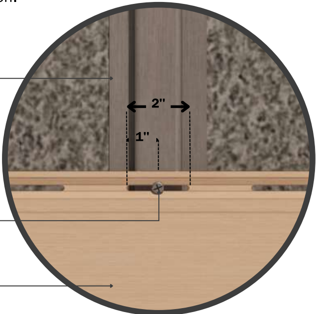
DETAIL Siding 6" & 4" Quik-Trim System
