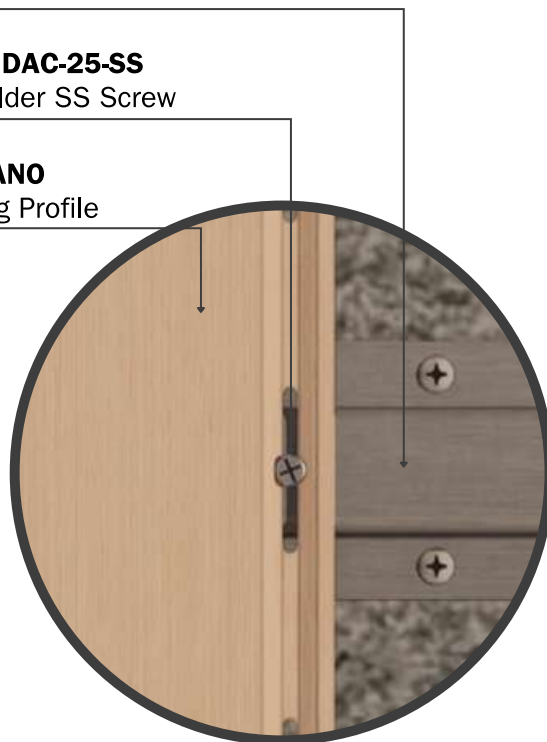
DETAIL B
