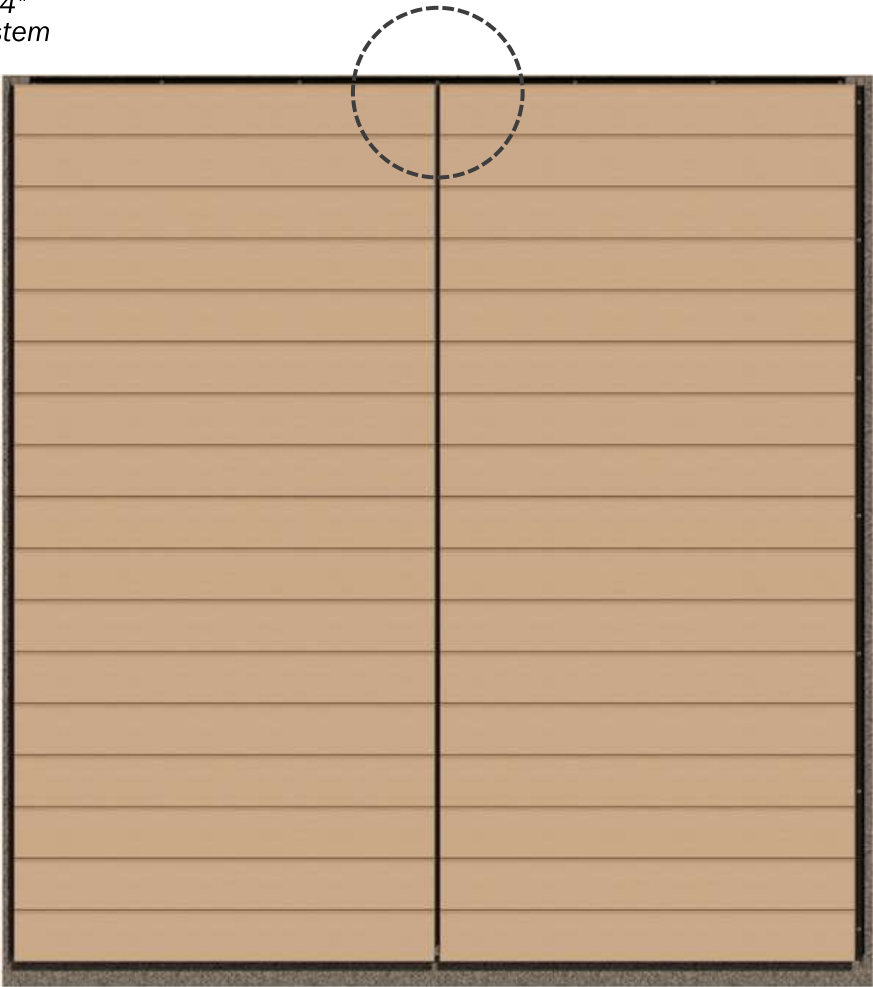
FRONT ELEVATION Siding 6" & 4" Quik-Trim System
