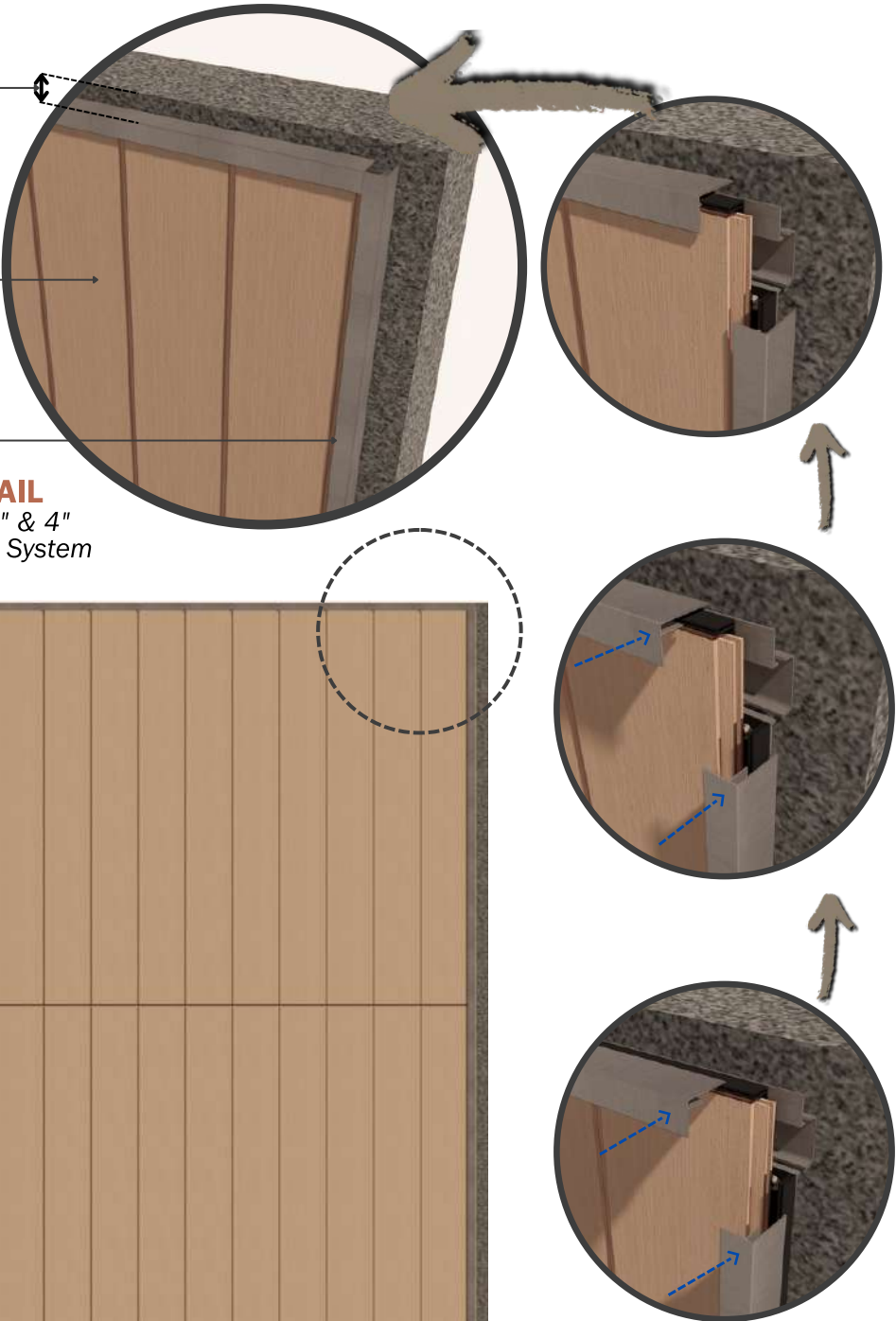
Install the Quik-Trim J-Mold & Quik-Trim Windows J-Mold into the PVC Base
