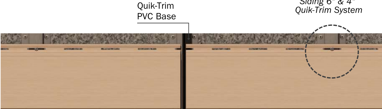
FRONT ELEVATION Siding 6" & 4" Quik-Trim System
