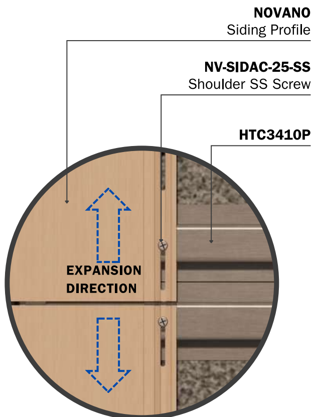
DETAIL A
