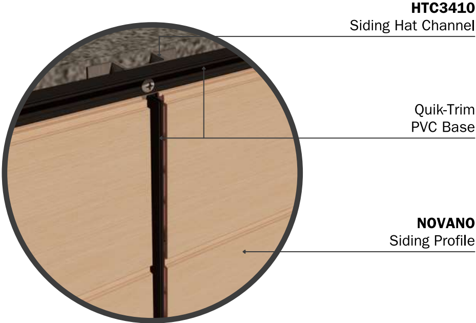
DETAIL Siding 6" & 4" Quik-Trim System
