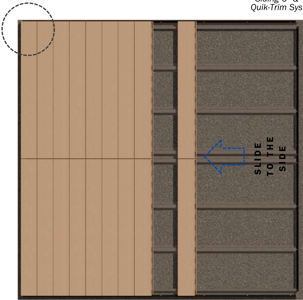
FRONT ELEVATION Siding 6" & 4" Quik-Trim System
