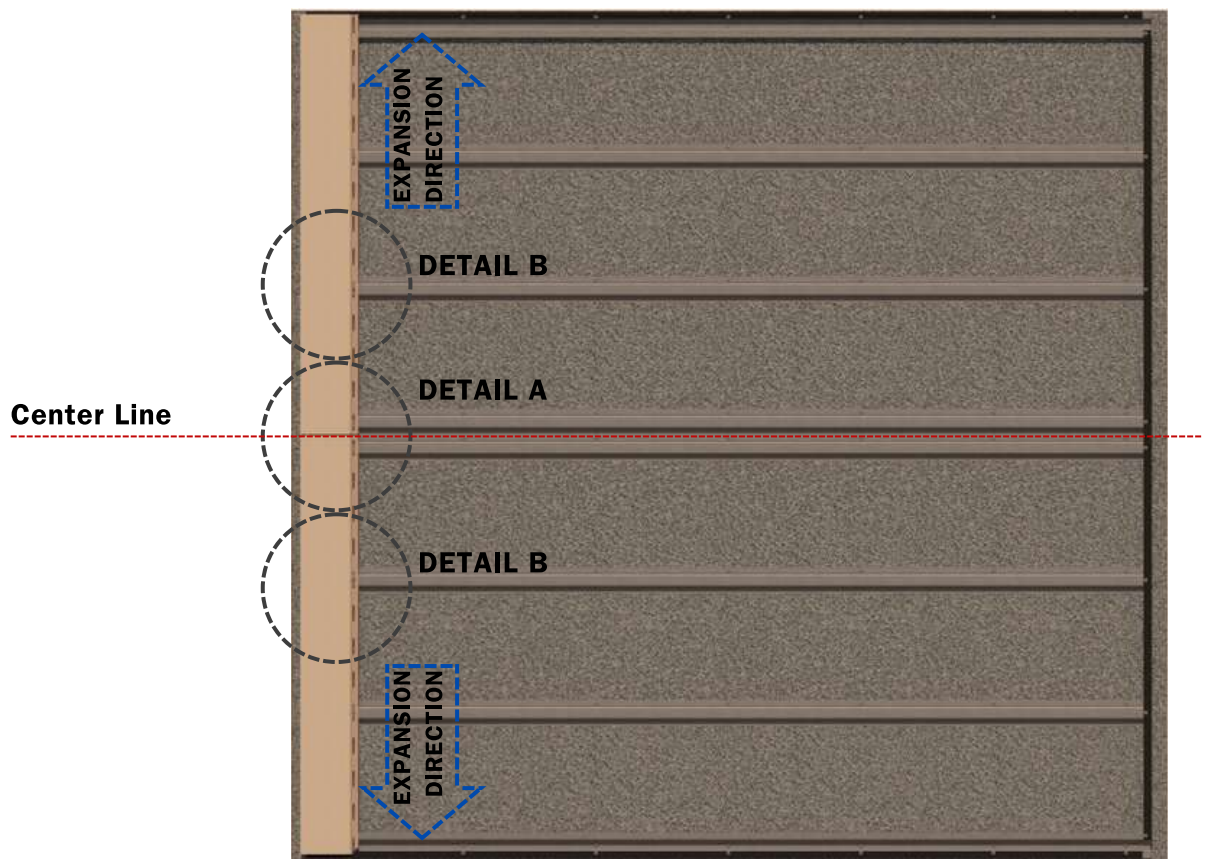
FRONT ELEVATION Siding 6" & 4" Quik-Trim System
