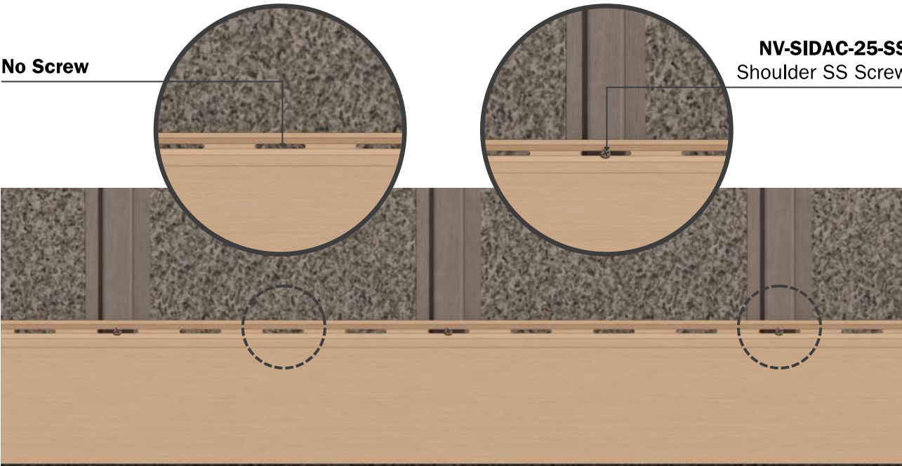
FRONT ELEVATION Siding 6" & 4" Quik-Trim System
