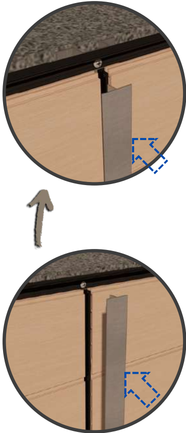
Install the H-Mold into the PVC Base
