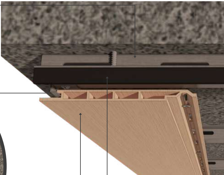
Quik-Trim PVC Base
