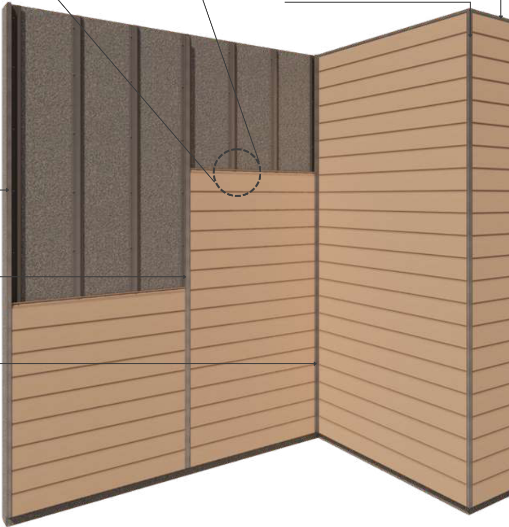
ISOMETRIC VIEW Basic Parts of Siding Board (Siding 6" & 4") Quik-Trim System
