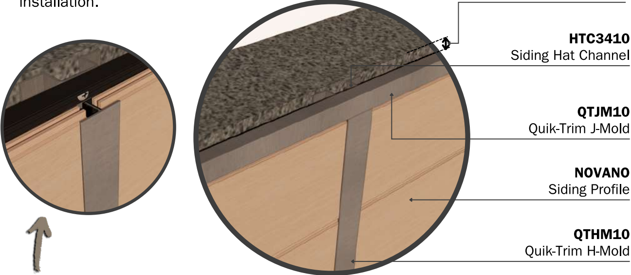
DETAIL Siding 6" & 4" Quik-Trim System
