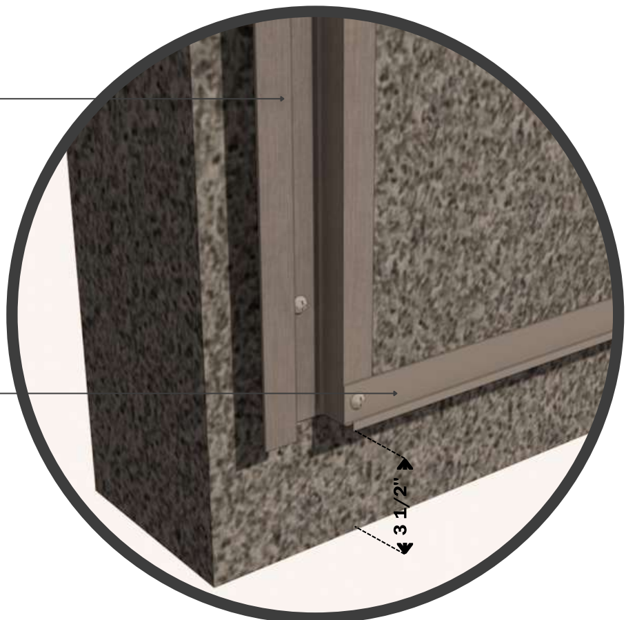
DETAIL Siding Starter J-Strip Siding 6" & 4" Quik-Trim System
